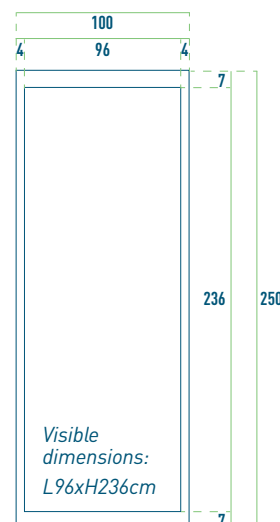
Technical layout of a wall
